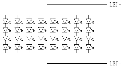
4*8=32 CIRCUIT DIAGRAM
